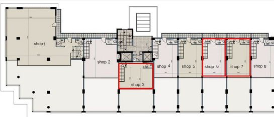
Plans – Shops Mezzanine Level
