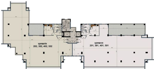
Plans – Offices: 2 nd , 3 rd , 4 th , 5 th Floor Level
